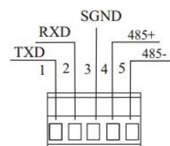
RS-232/485 input interface
